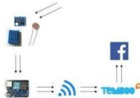
Gambar 2. Diagram Blok
