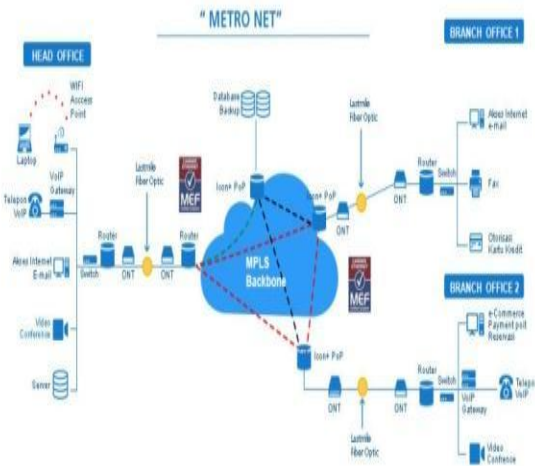
Gambar 4. Topologi Metronet
