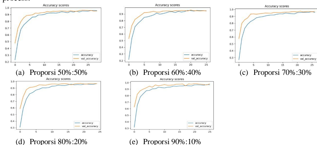
Figure 3. Accuracy Graph Result of MobileNetV2 Method
