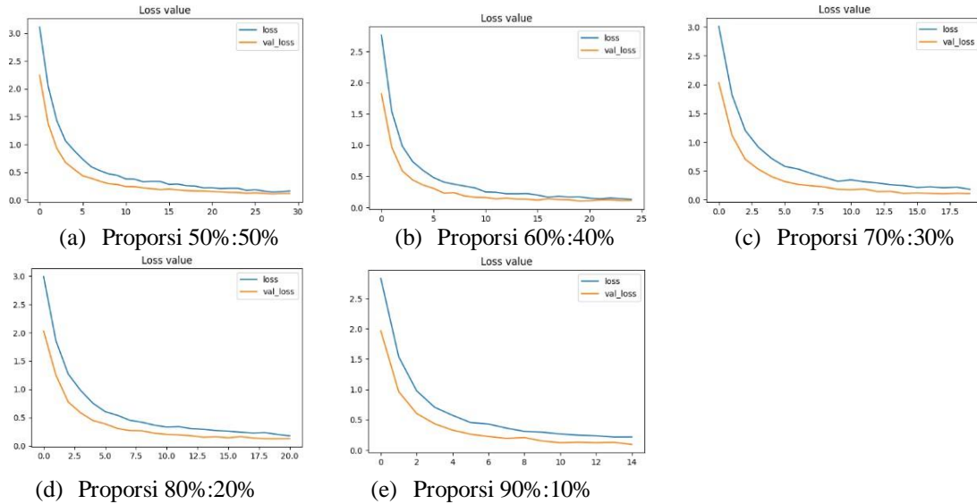
Figure 6. Loss Graph Results of ResNet50V2 Method
