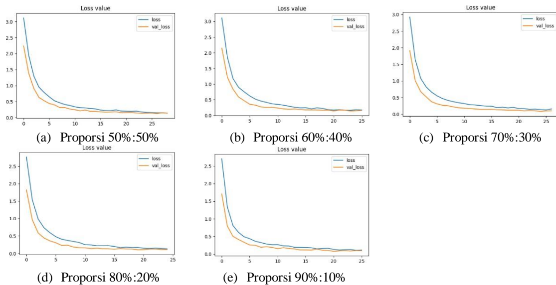
Figure 4. Loss Graph Results of MobileNetV2 Method
