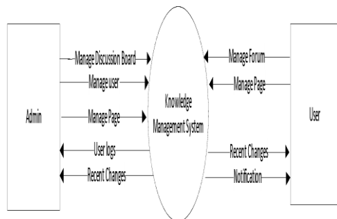
Gambar 4. Diagram context
