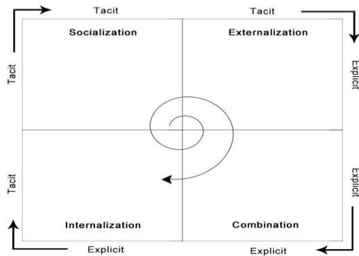
Gambar 1. SECI Model [7]
