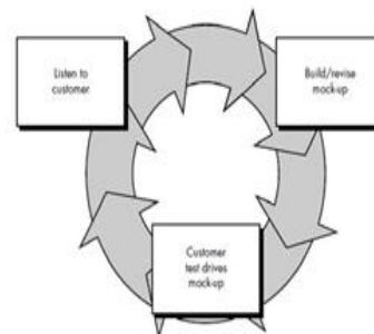
Gambar 3. Prototyping Model [12]
