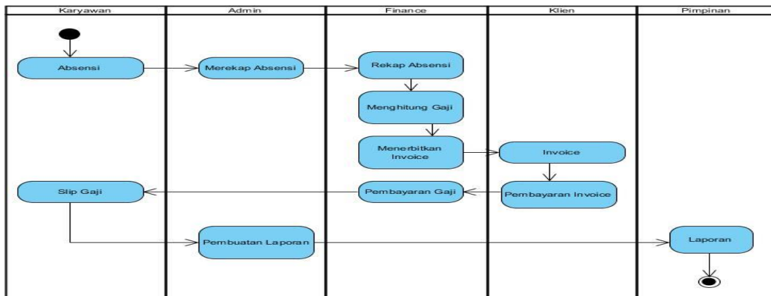
Figure 2. Activity Diagram
