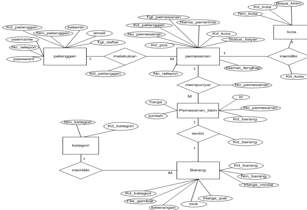
Gambar 2. ERD (Entity Relationship Diagram)
