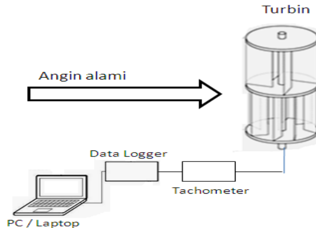
Gambar 2. Instalasi Penelitian
