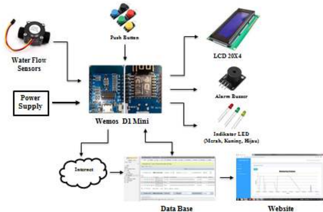
Gambar 4. Diagram Blok
