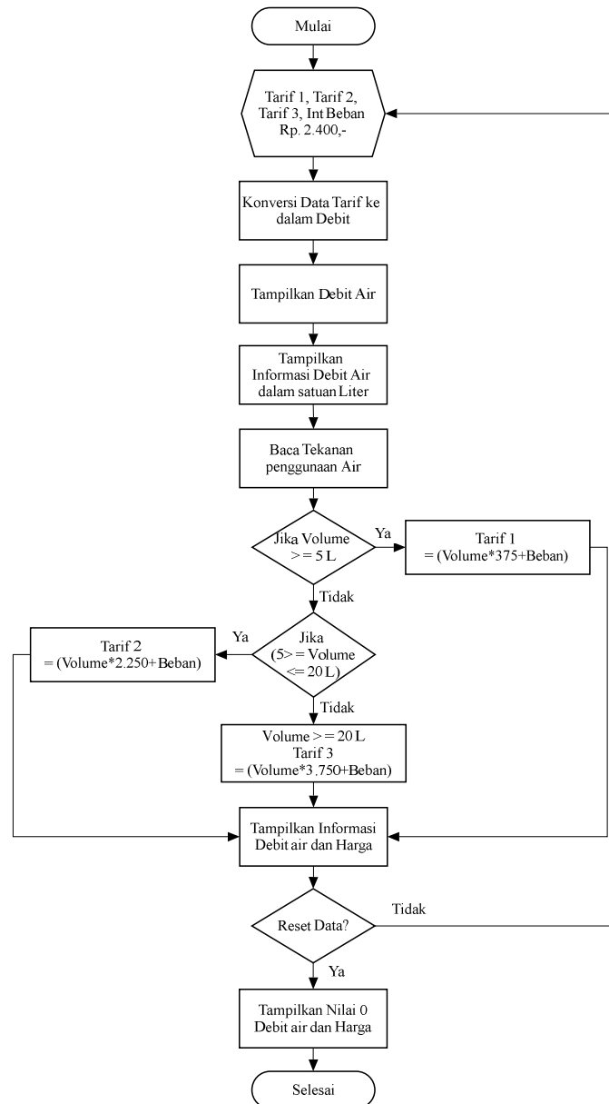
Gambar 7. Flowchart Sistem
