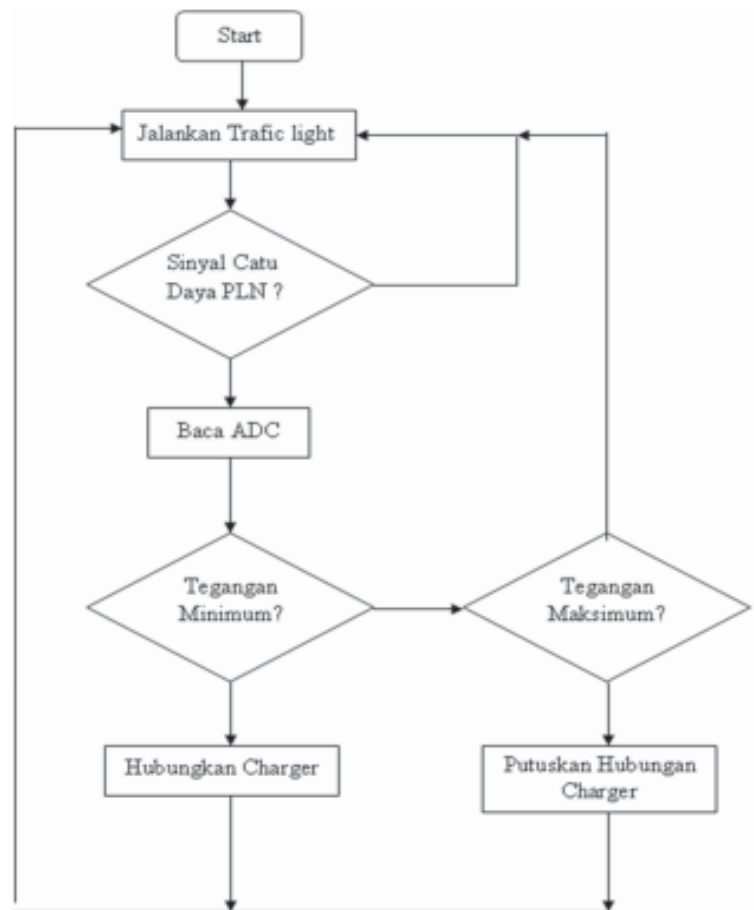
Gambar 11. Flowchart
