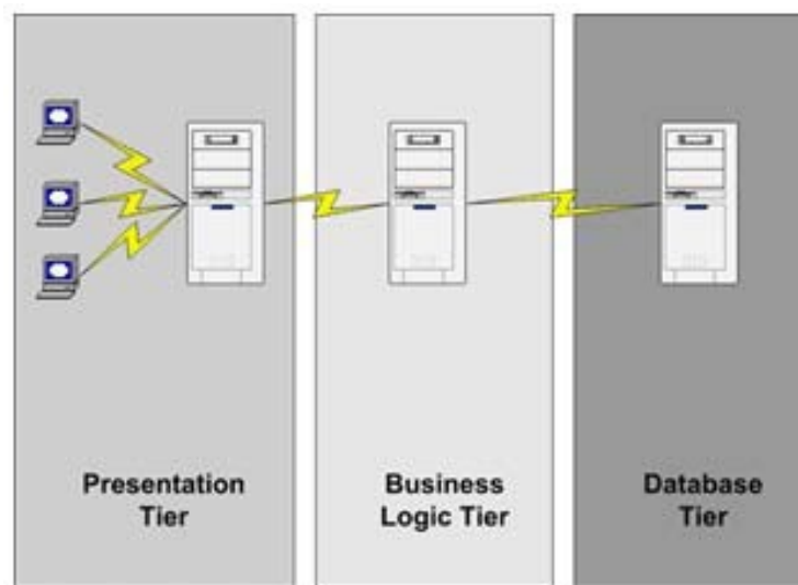
Gambar 5. Architecture Three-Tier
