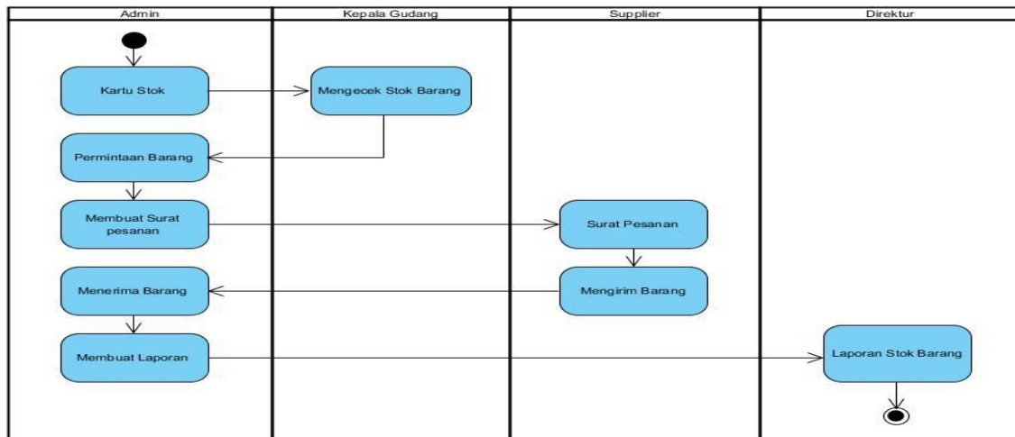
Gambar 2. Activity Diagram
