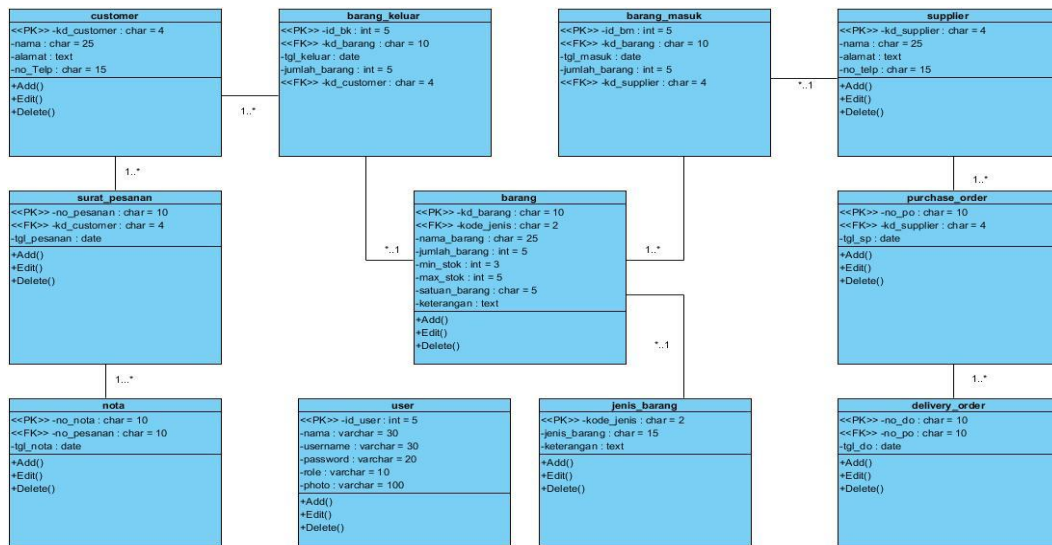
Gambar 4. Class Diagram
